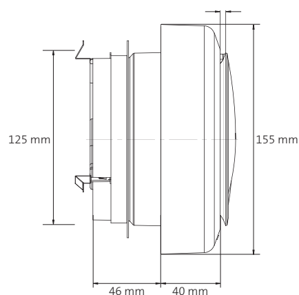
Supply valve, DN125 (■ = recommended application range)
