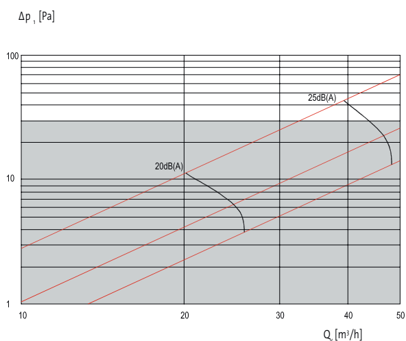
Supply valve, DN125 (■ = recommended application range)
